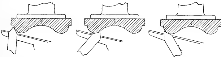
FIG. 323. CONVEX SCRAPING WITH SPEAR-POINT CHISEL.
